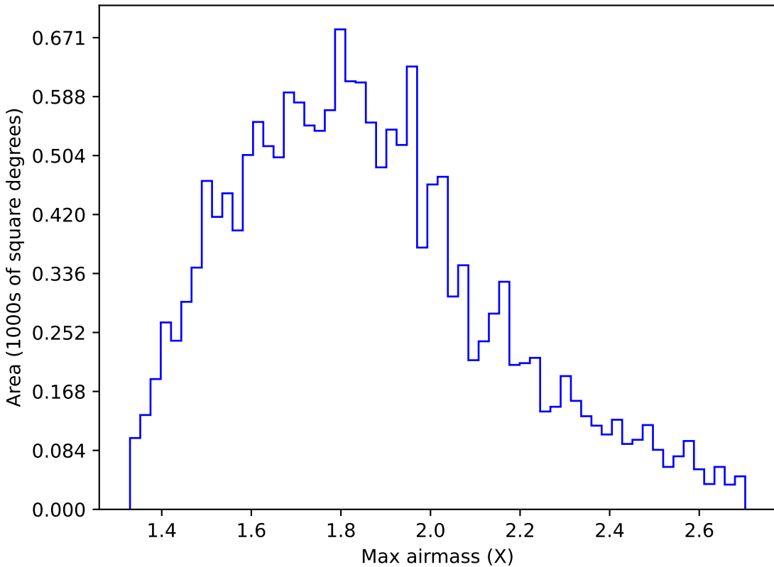
extra_ss_neo4_v3.4_10yrs WFD u band: Max airmass
