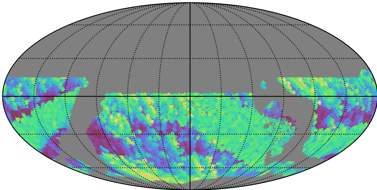
extra_ss_neo4_v3.4_10yrs WFD r band: Max airmass
