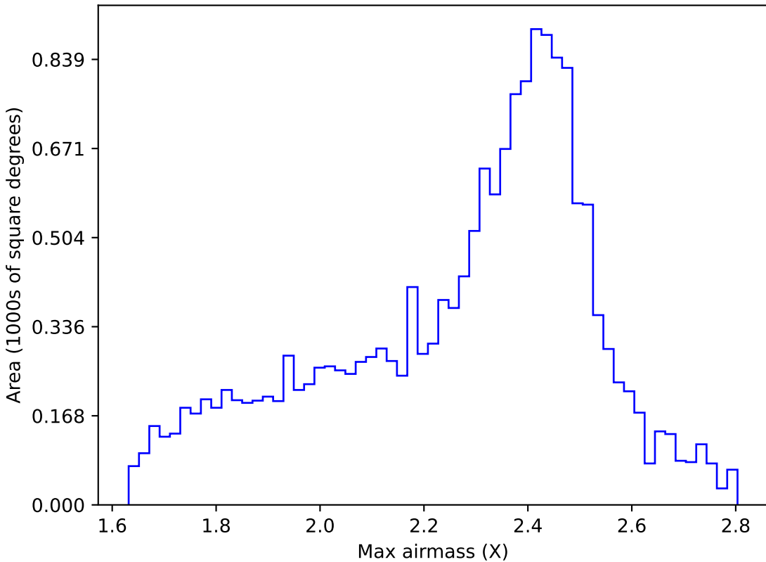
extra_ss_neo4_v3.4_10yrs WFD r band: Max airmass
