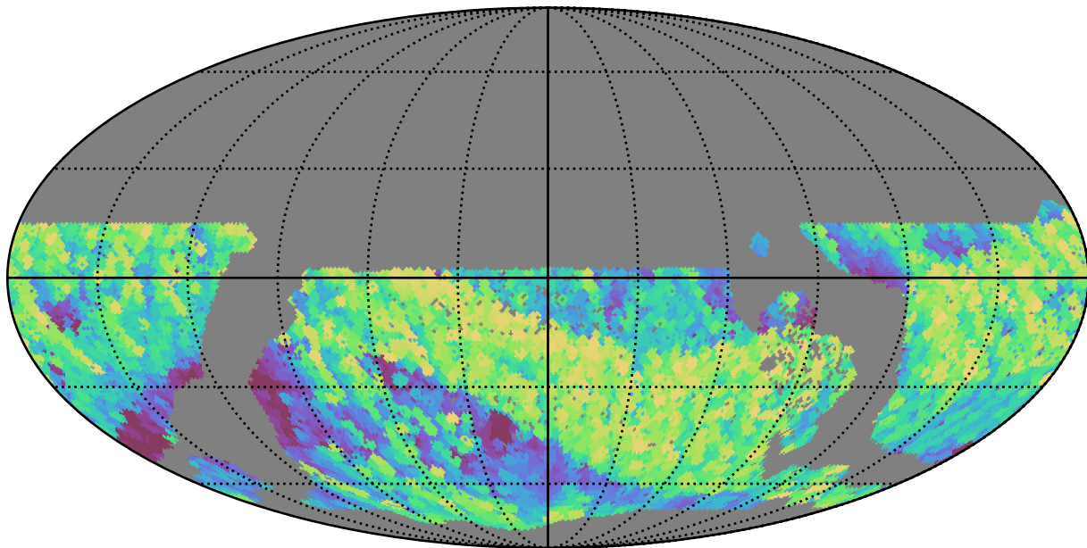
extra_ss_neo4_v3.4_10yrs WFD i band: Max airmass
