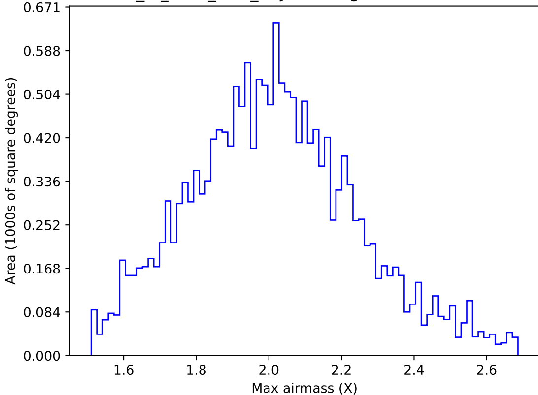
extra_ss_neo4_v3.4_10yrs WFD g band: Max airmass
