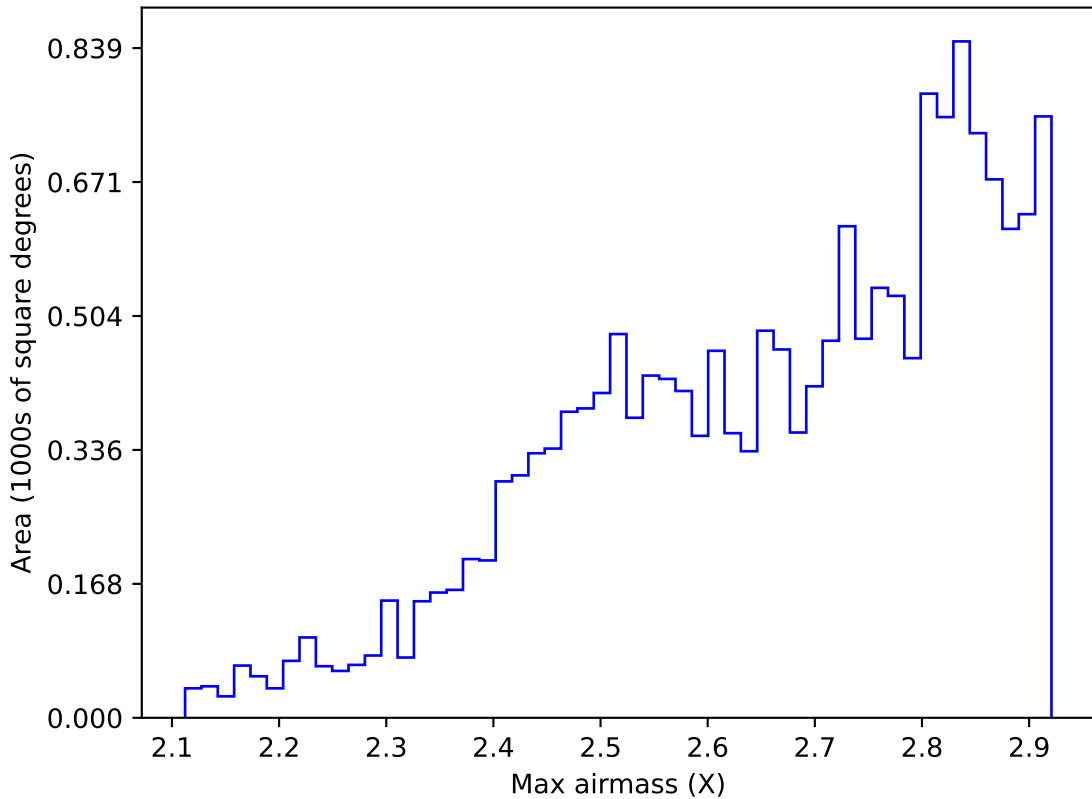
extra_ss_neo4_v3.4_10yrs WFD all bands: Max airmass
