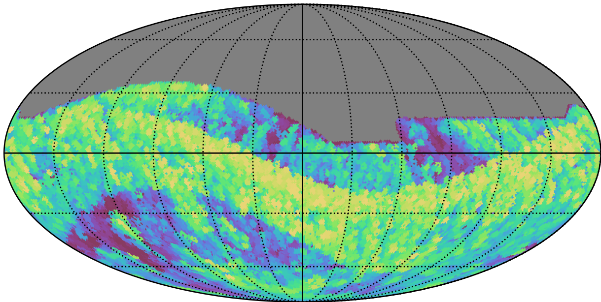
extra_ss_neo4_v3.4_10yrs All sky z band: Max airmass
