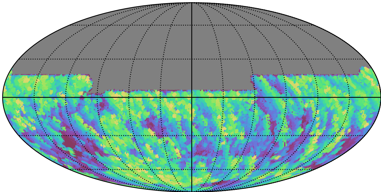
extra_ss_neo4_v3.4_10yrs All sky y band: Max airmass
