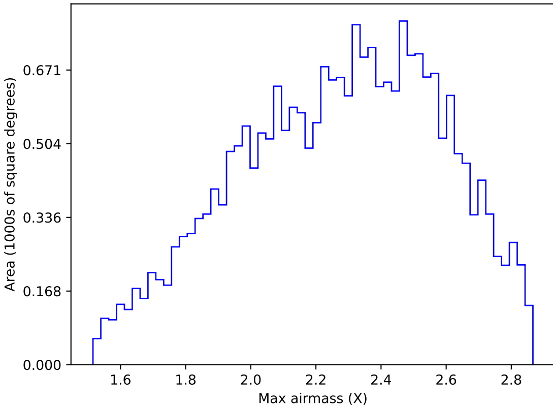
extra_ss_neo4_v3.4_10yrs All sky y band: Max airmass
