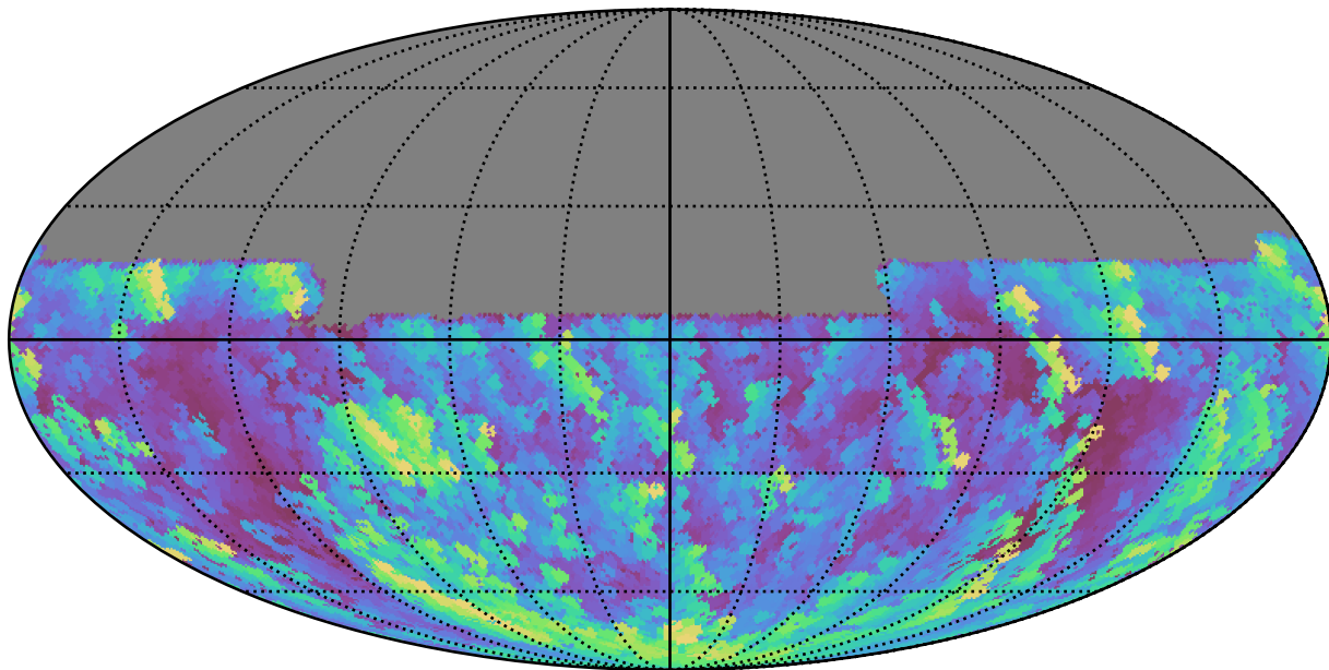
extra_ss_neo4_v3.4_10yrs All sky u band: Max airmass
