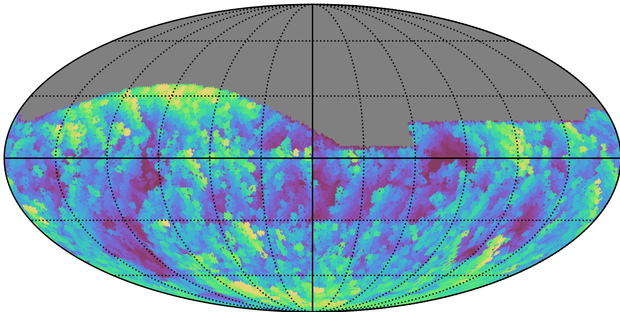
extra_ss_neo4_v3.4_10yrs All sky g band: Max airmass
