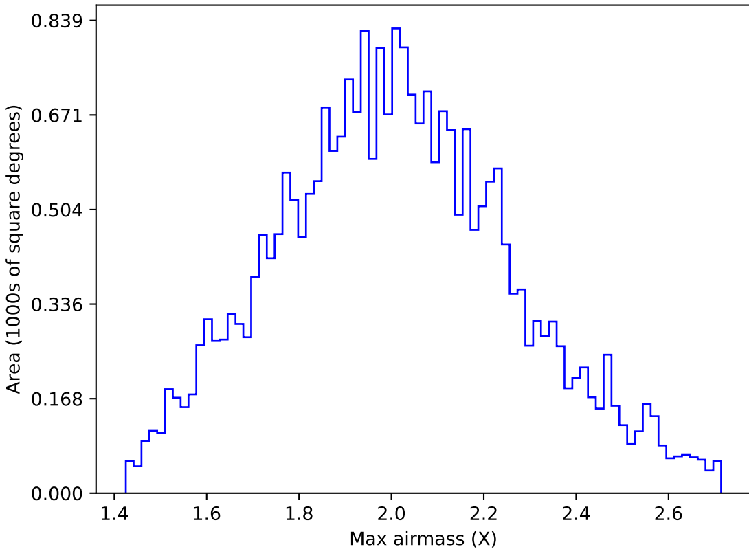
extra_ss_neo4_v3.4_10yrs All sky g band: Max airmass
