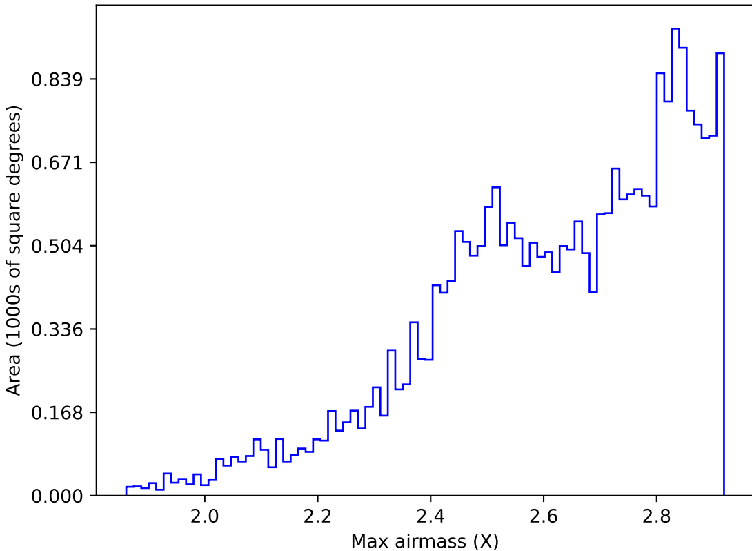
extra_ss_neo4_v3.4_10yrs All sky all bands: Max airmass
