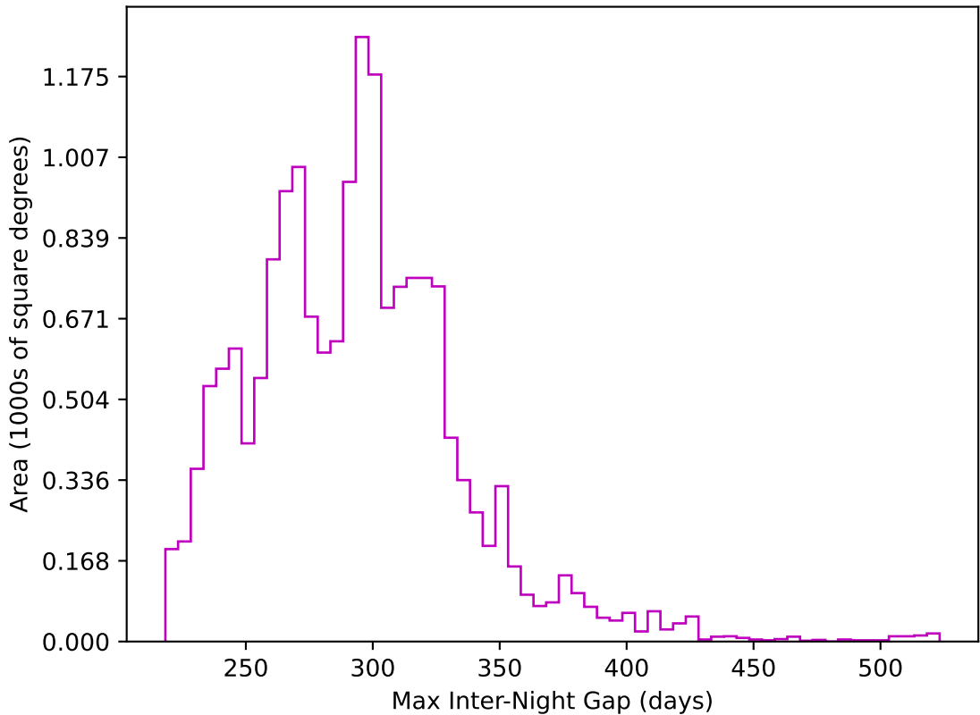
extra_ss_neo4_v3.4_10yrs WFD z band: Max Inter-Night Gap
