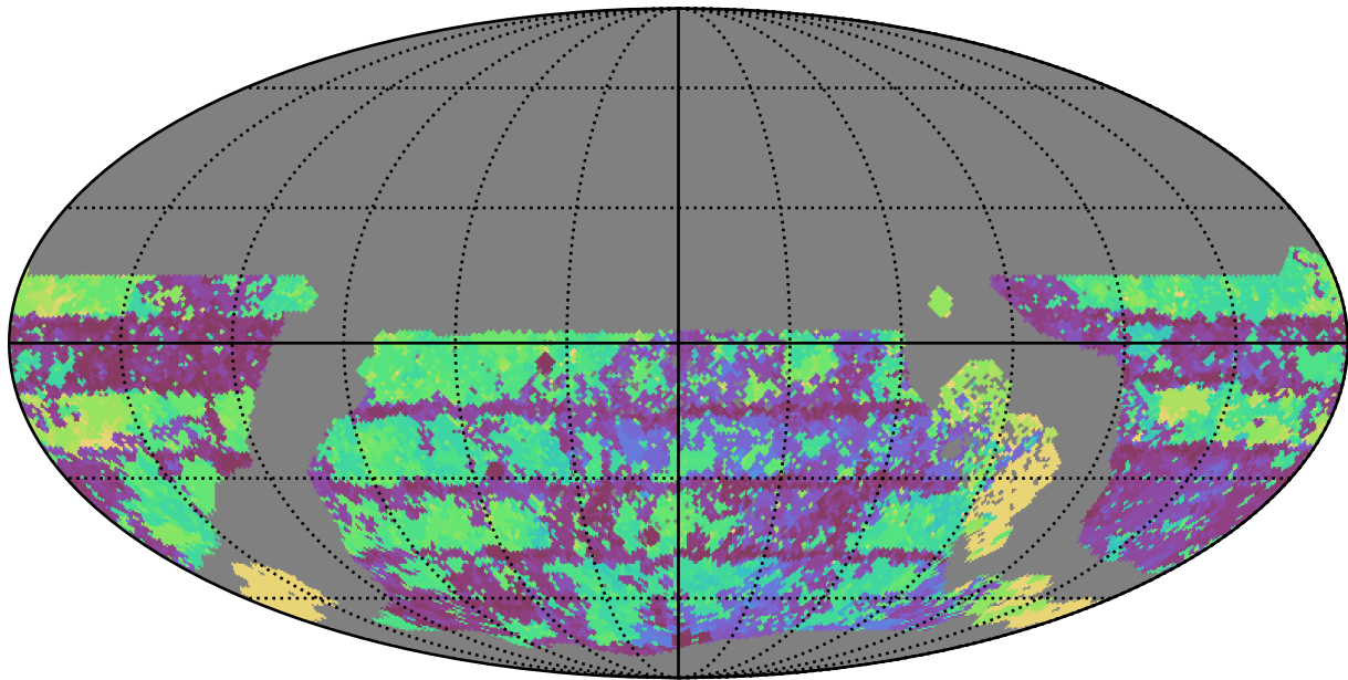
extra_ss_neo4_v3.4_10yrs WFD u band: Max Inter-Night Gap
