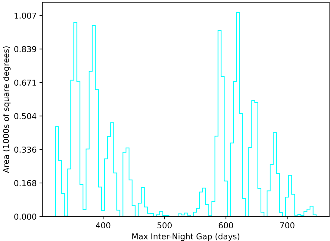
extra_ss_neo4_v3.4_10yrs WFD u band: Max Inter-Night Gap
