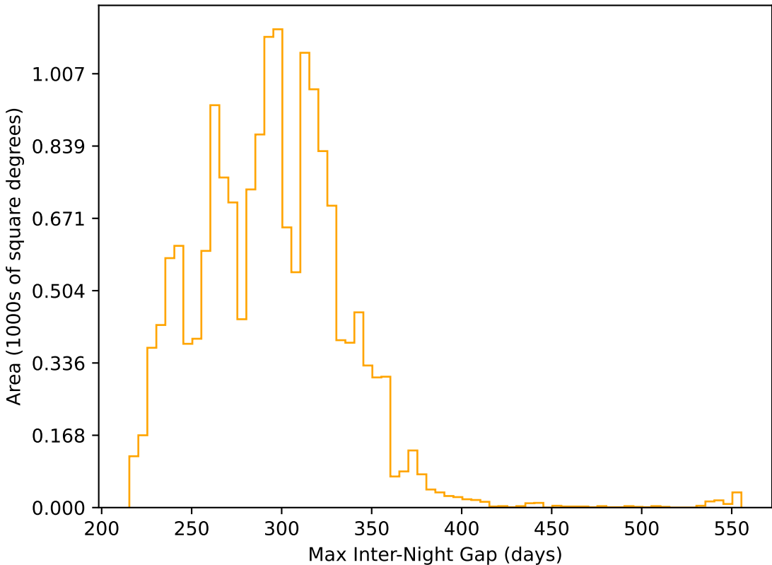
extra_ss_neo4_v3.4_10yrs WFD r band: Max Inter-Night Gap
