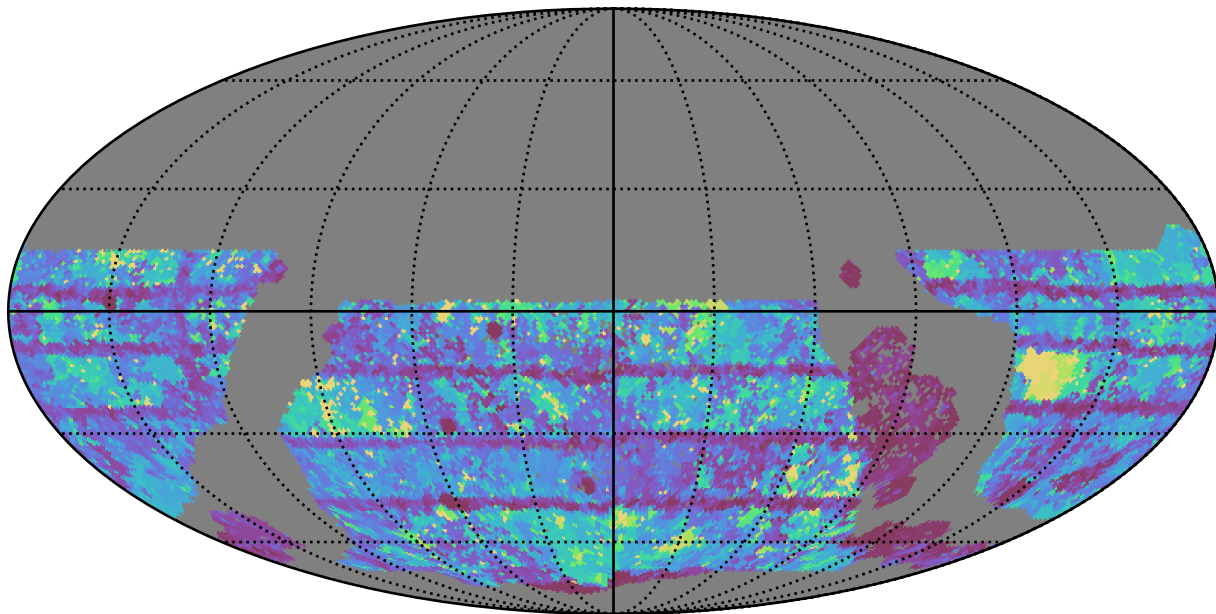
extra_ss_neo4_v3.4_10yrs WFD i band: Max Inter-Night Gap
