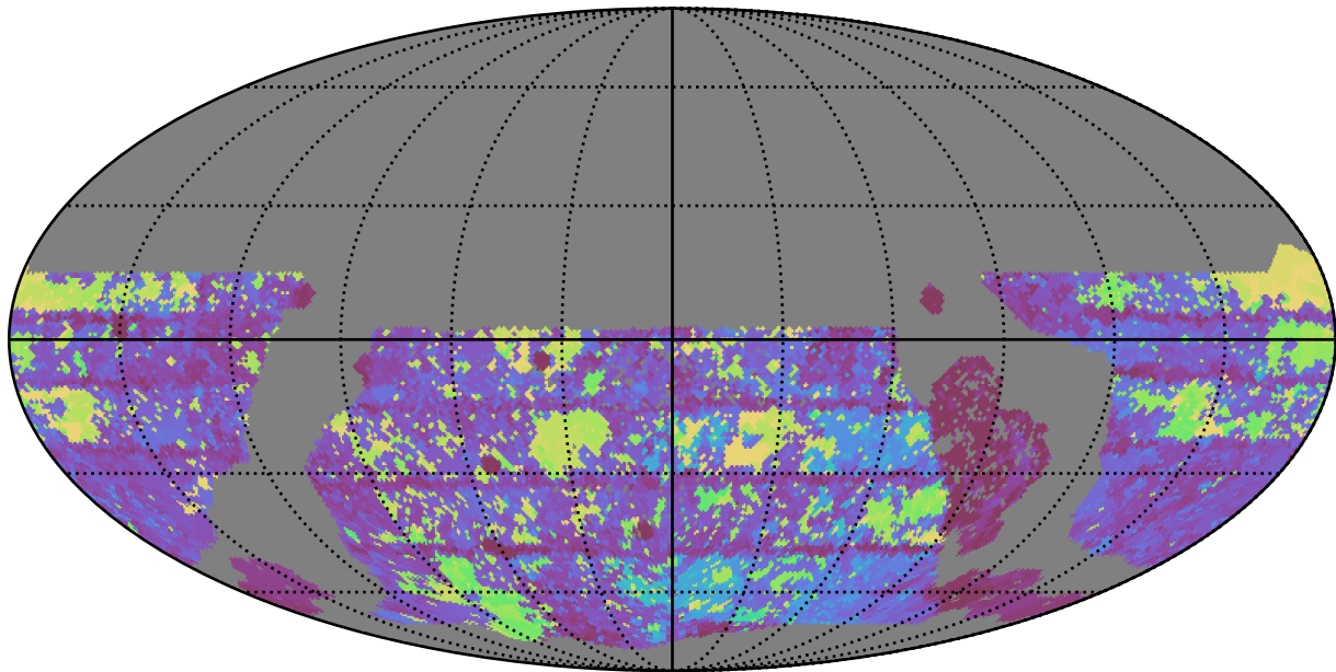
extra_ss_neo4_v3.4_10yrs WFD g band: Max Inter-Night Gap
