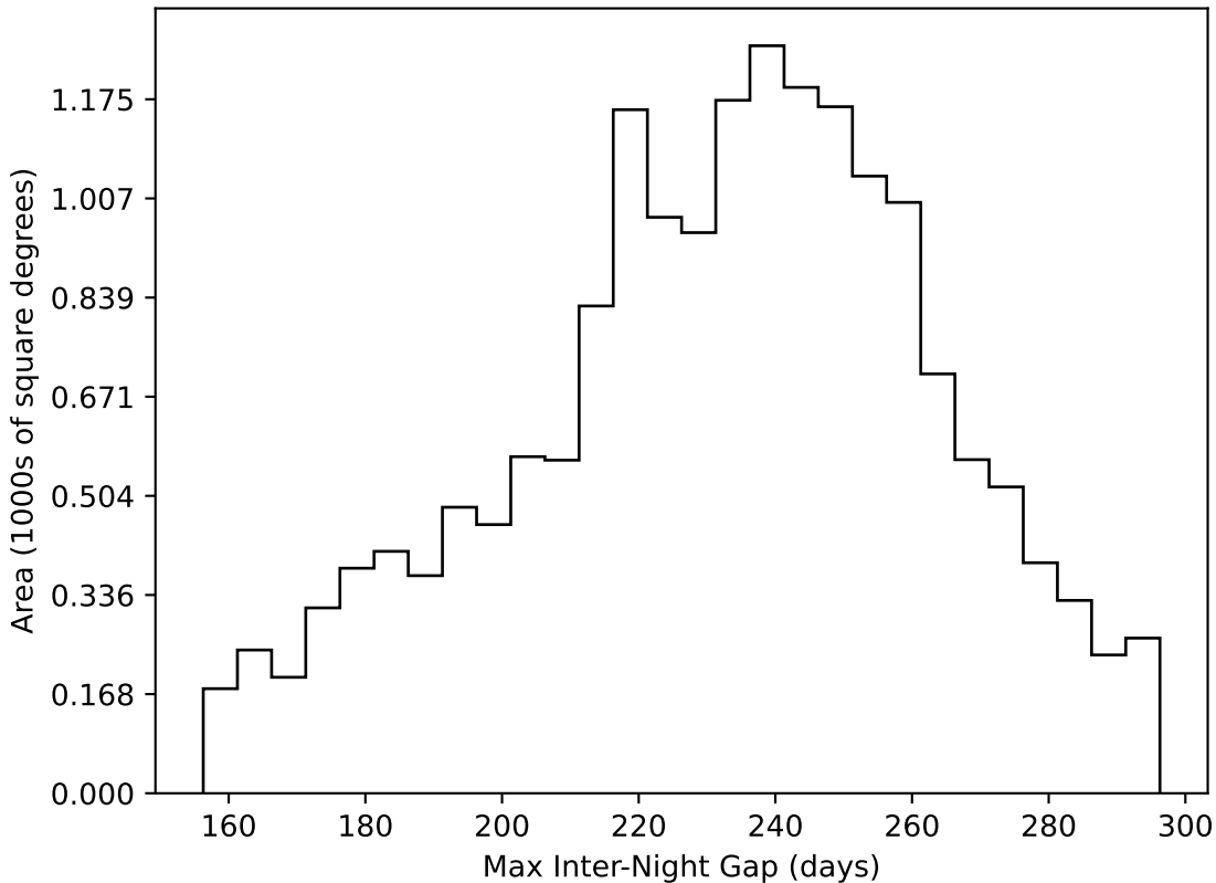
extra_ss_neo4_v3.4_10yrs WFD all bands: Max Inter-Night Gap
