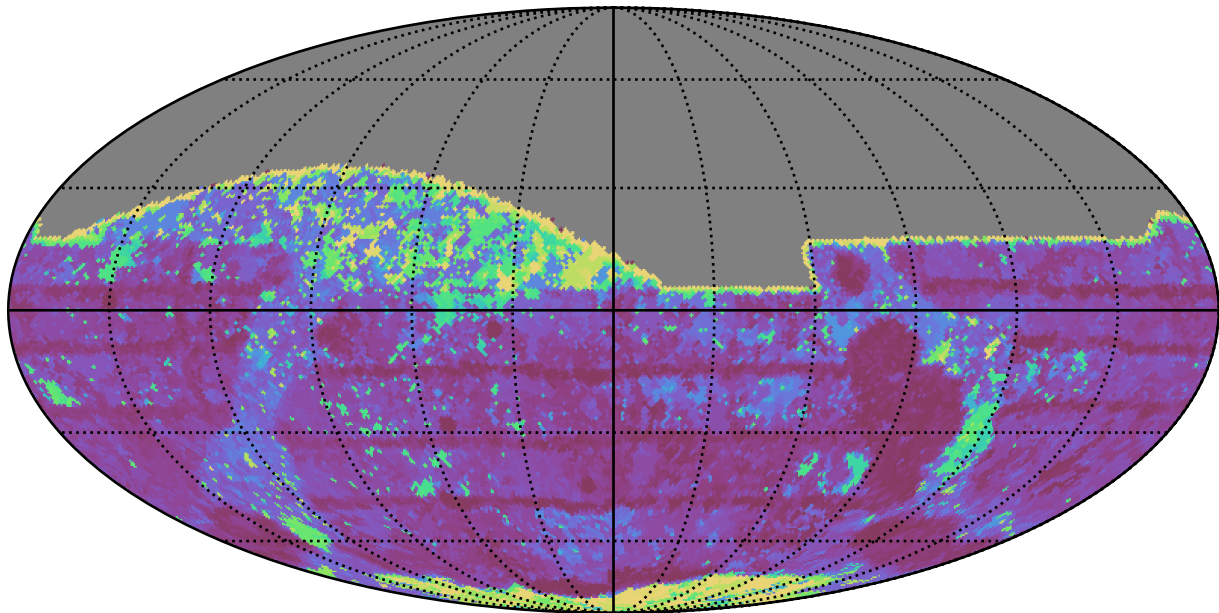
extra_ss_neo4_v3.4_10yrs All sky z band: Max Inter-Night Gap
