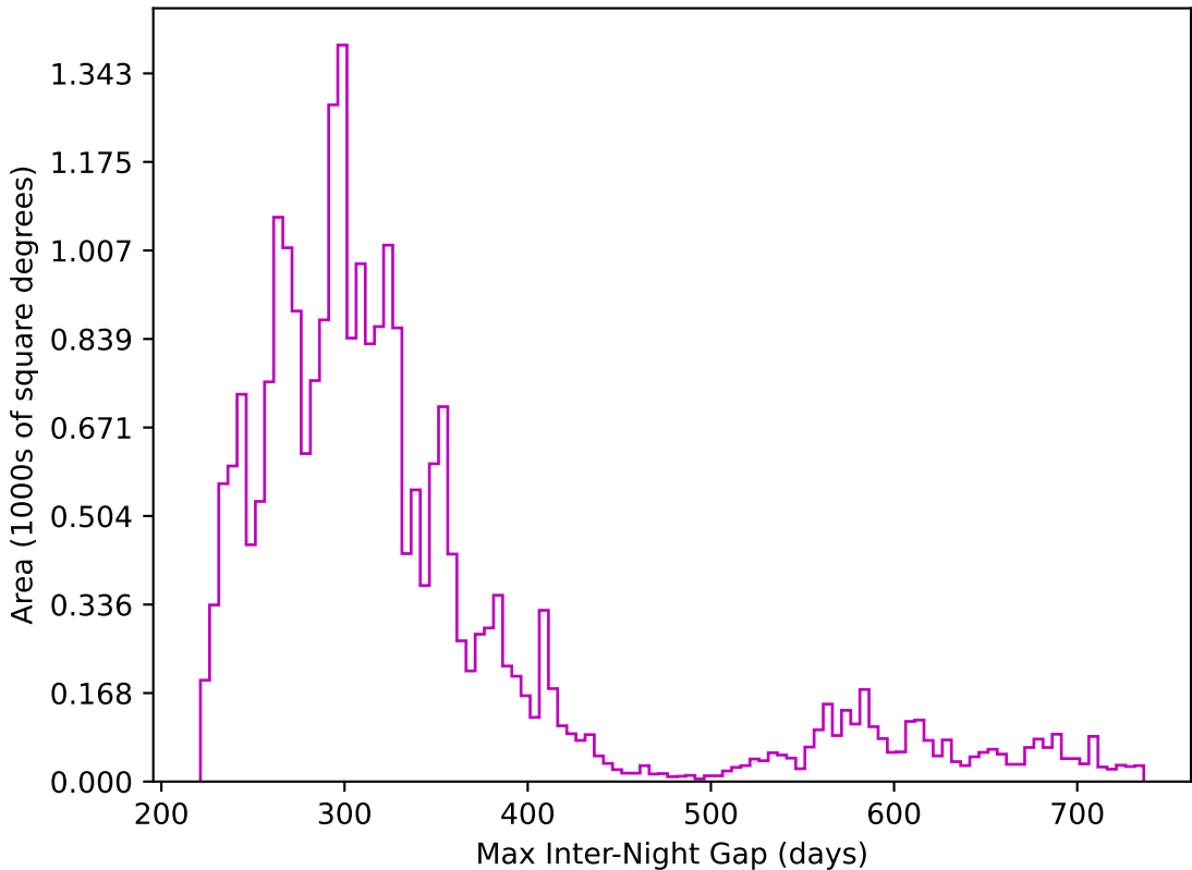
extra_ss_neo4_v3.4_10yrs All sky z band: Max Inter-Night Gap
