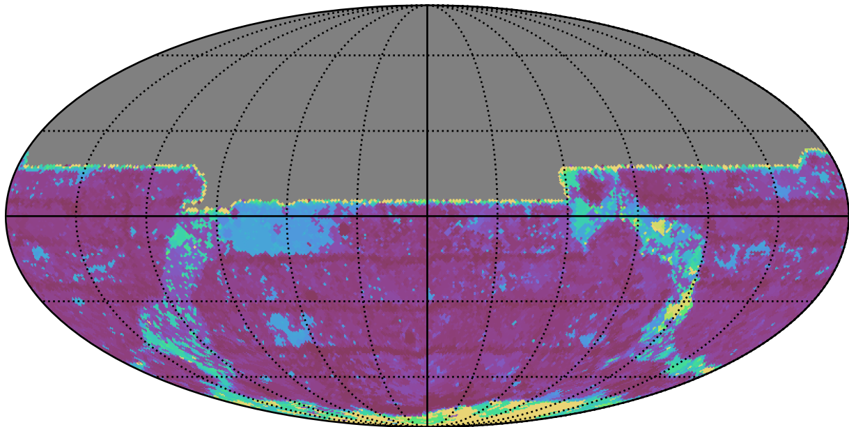
extra_ss_neo4_v3.4_10yrs All sky y band: Max Inter-Night Gap
