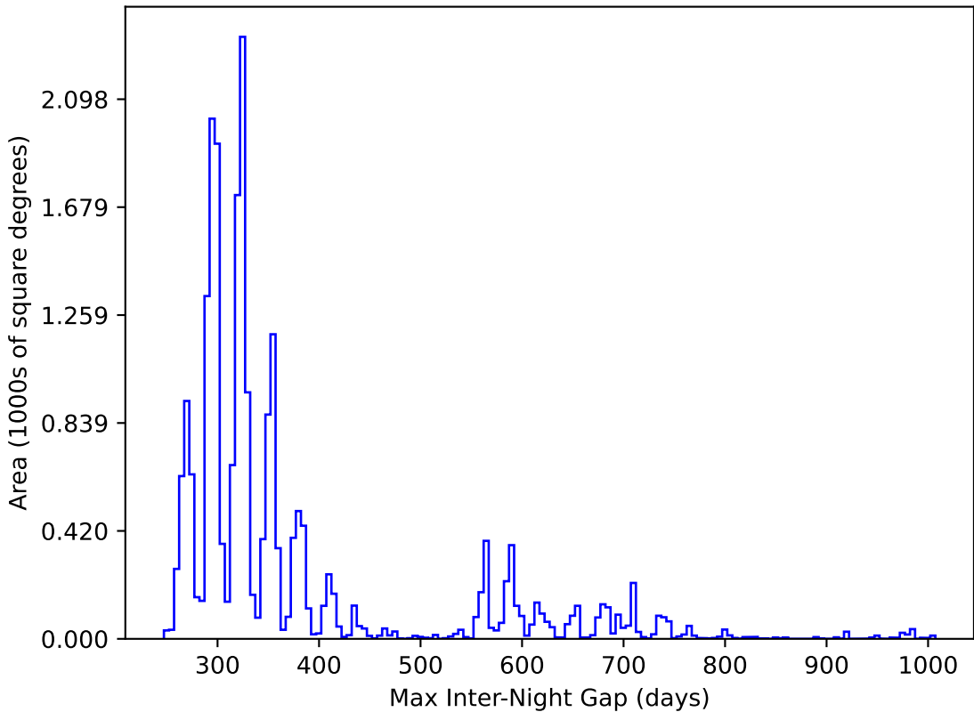
extra_ss_neo4_v3.4_10yrs All sky y band: Max Inter-Night Gap
