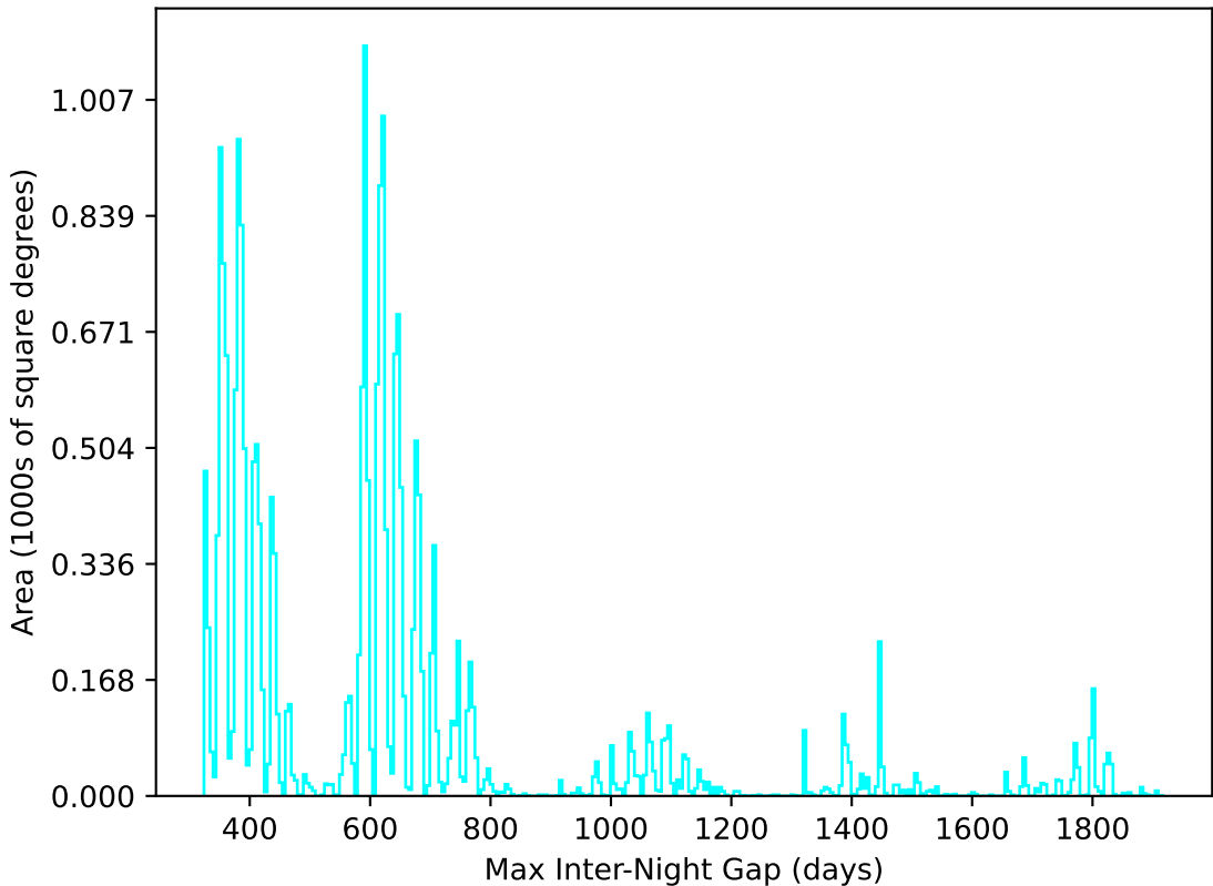
extra_ss_neo4_v3.4_10yrs All sky u band: Max Inter-Night Gap
