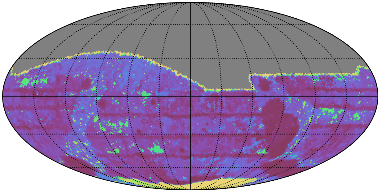
extra_ss_neo4_v3.4_10yrs All sky r band: Max Inter-Night Gap
