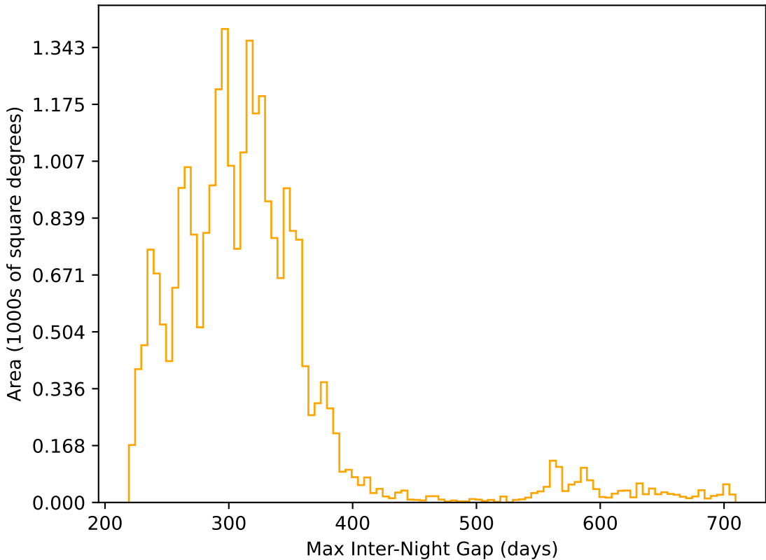
extra_ss_neo4_v3.4_10yrs All sky r band: Max Inter-Night Gap
