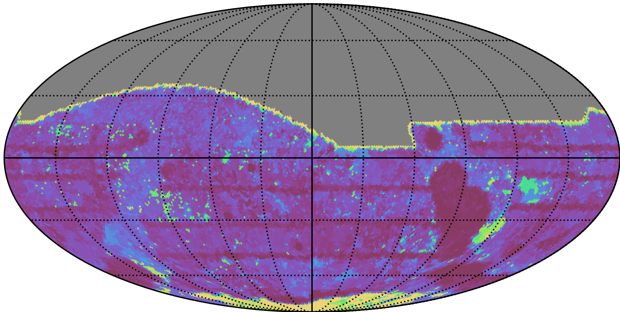
extra_ss_neo4_v3.4_10yrs All sky i band: Max Inter-Night Gap
