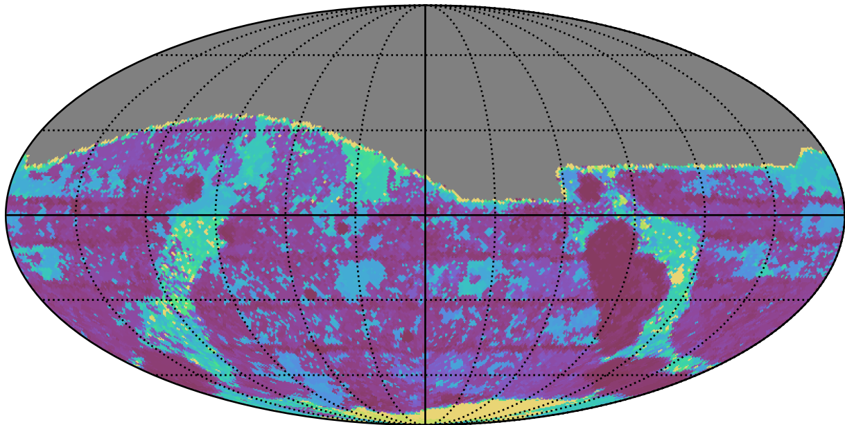
extra_ss_neo4_v3.4_10yrs All sky g band: Max Inter-Night Gap
