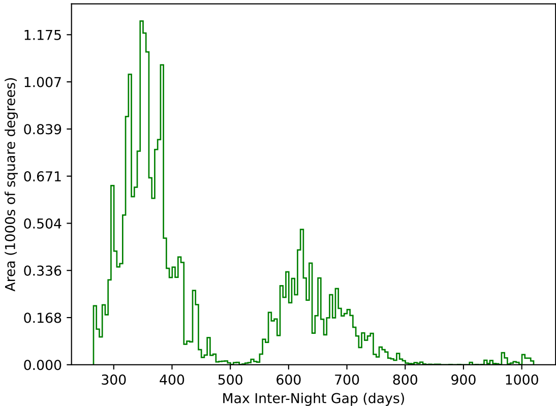
extra_ss_neo4_v3.4_10yrs All sky g band: Max Inter-Night Gap
