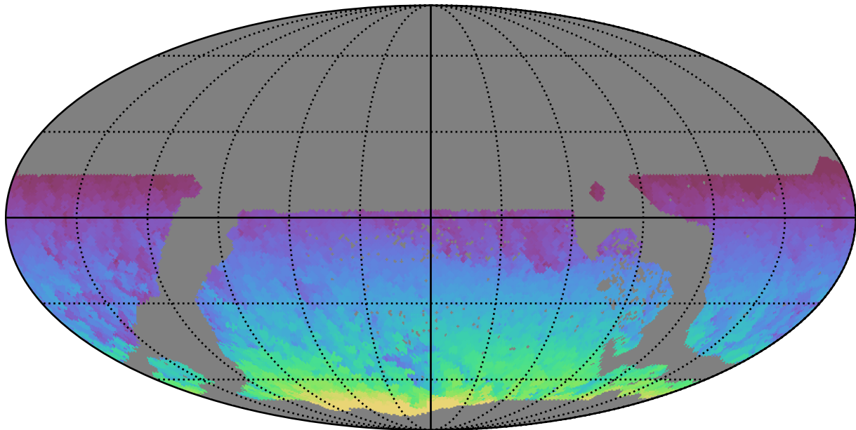
extra_ss_neo4_v3.4_10yrs WFD all bands: Max HA
