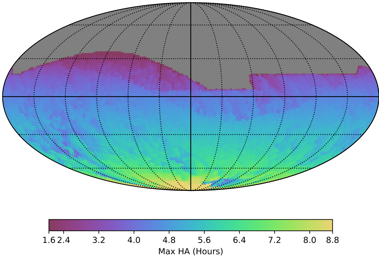
extra_ss_neo4_v3.4_10yrs All sky all bands: Max HA
