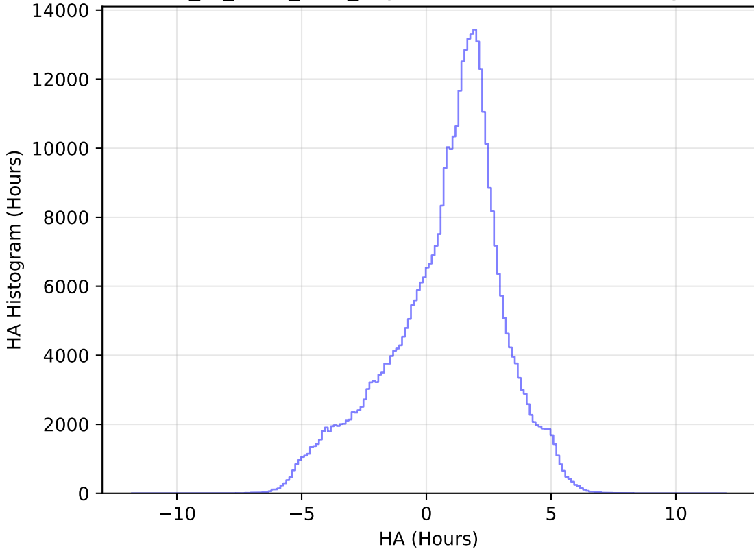
extra_ss_neo4_v3.4_10yrs WFD z band: HA Histogram
