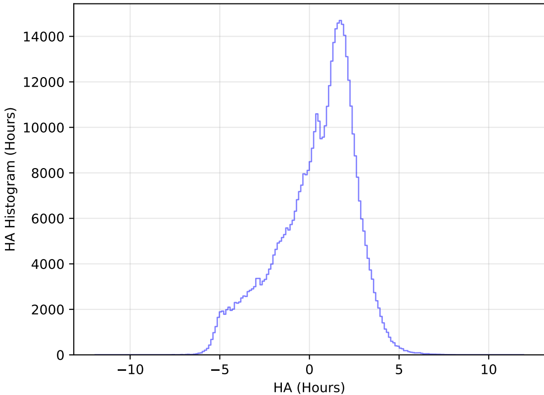
extra_ss_neo4_v3.4_10yrs WFD r band: HA Histogram
