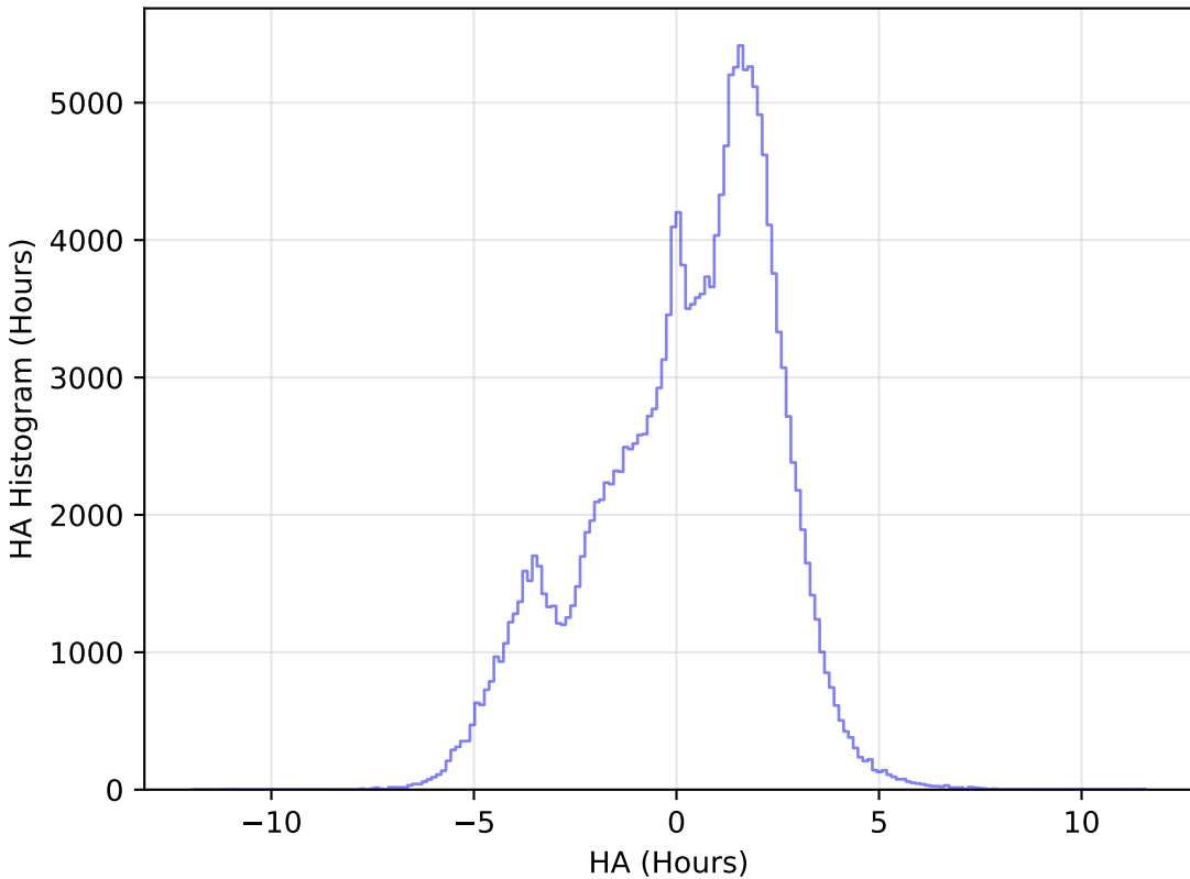
extra_ss_neo4_v3.4_10yrs WFD g band: HA Histogram
