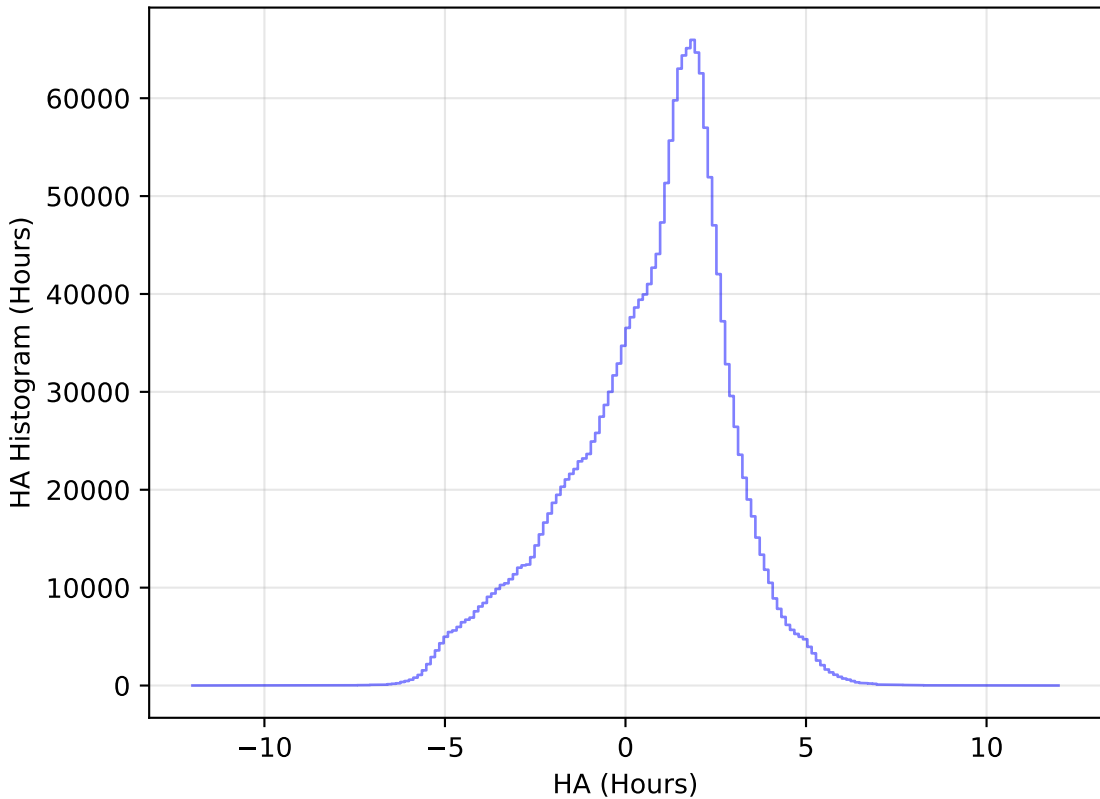
extra_ss_neo4_v3.4_10yrs All sky all bands: HA Histogram
