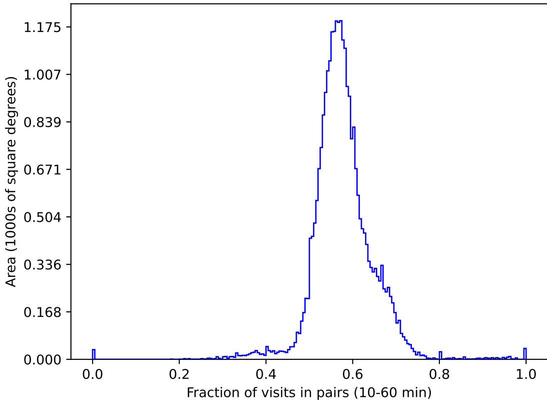
extra_ss_neo4_v3.4_10yrs gri All sky: Fraction of visits in pairs (10-60 min)
