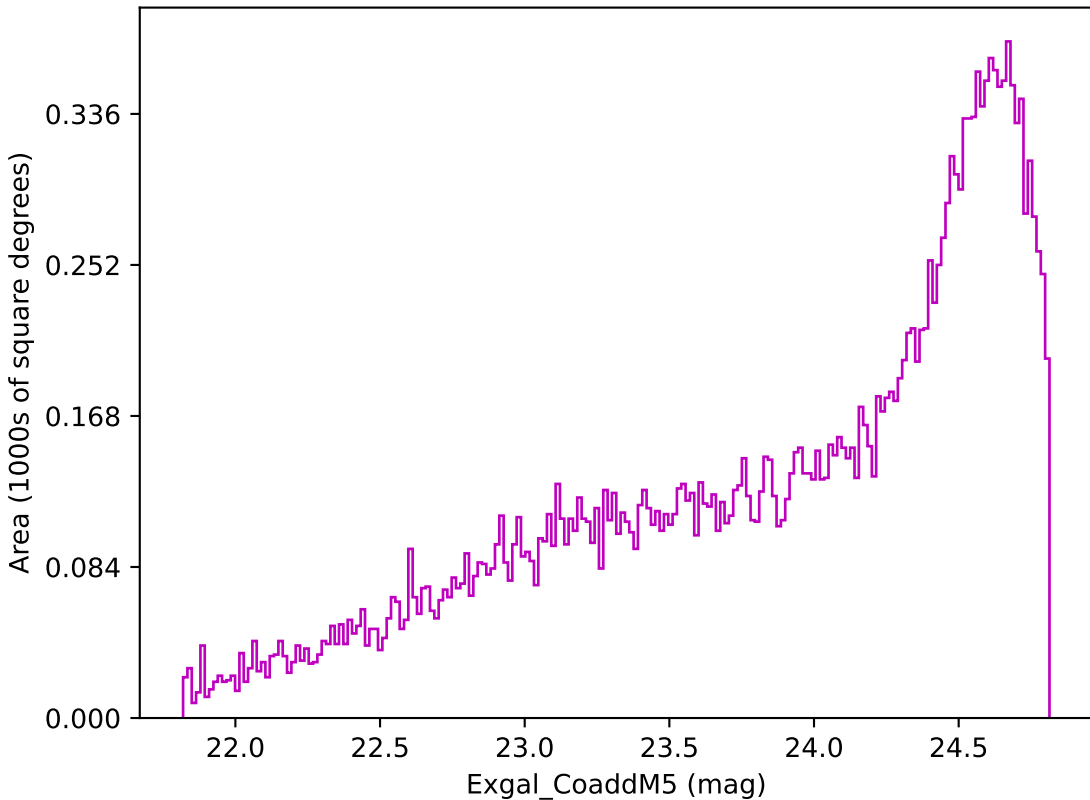
extra_ss_neo4_v3.4_10yrs Yr 3-4 z band: Exgal_CoaddM5
