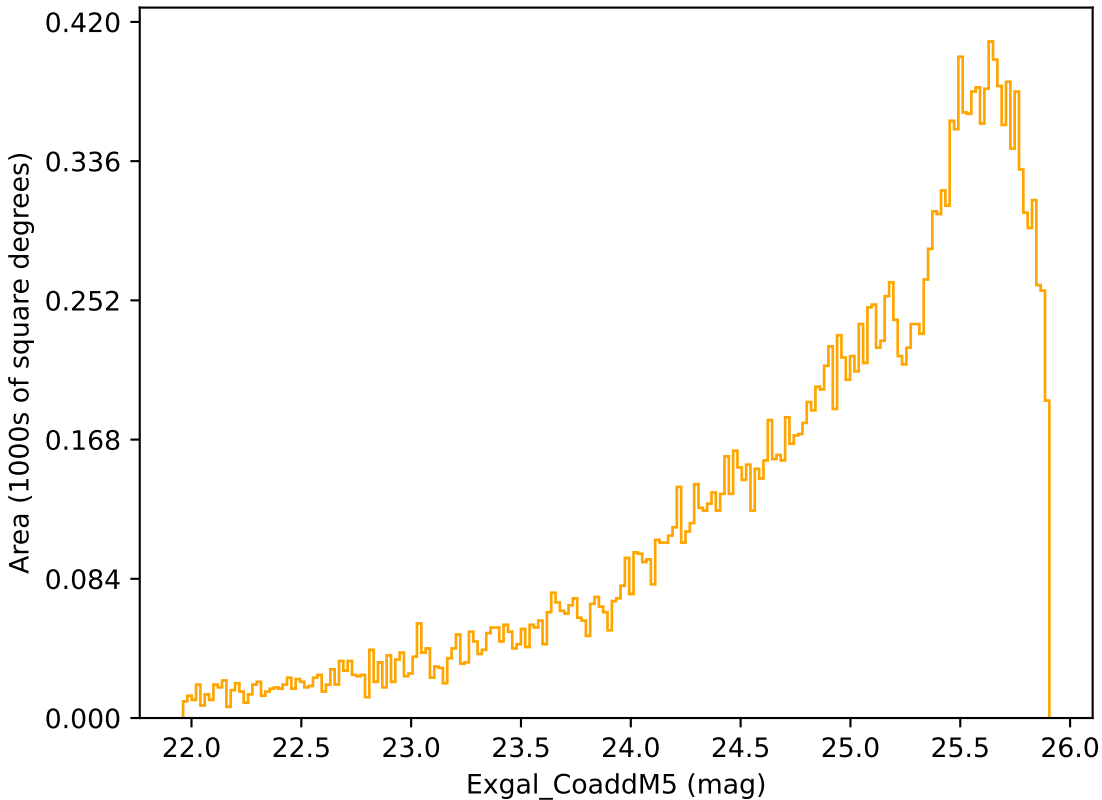
extra_ss_neo4_v3.4_10yrs Yr 3-4 r band: Exgal_CoaddM5
