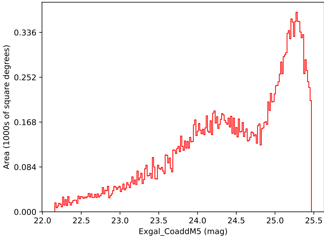
extra_ss_neo4_v3.4_10yrs Yr 3-4 i band: Exgal_CoaddM5
