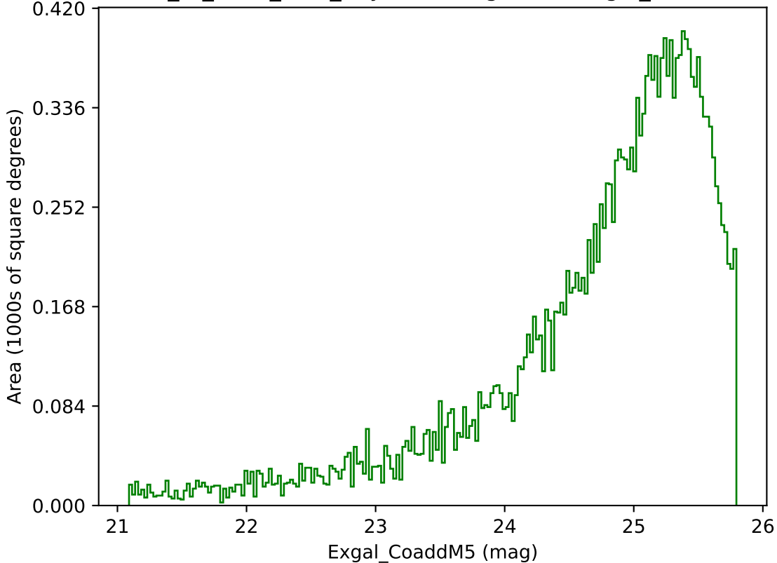
extra_ss_neo4_v3.4_10yrs Yr 3-4 g band: Exgal_CoaddM5
