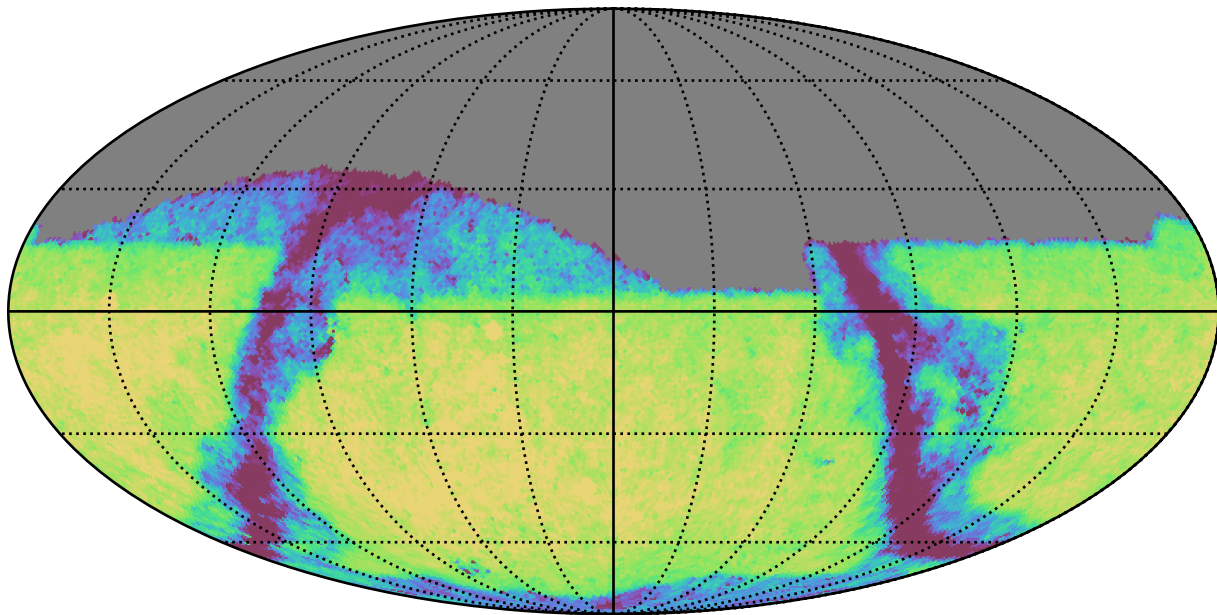
extra_ss_neo4_v3.4_10yrs Yr 1 z band: Exgal_CoaddM5
