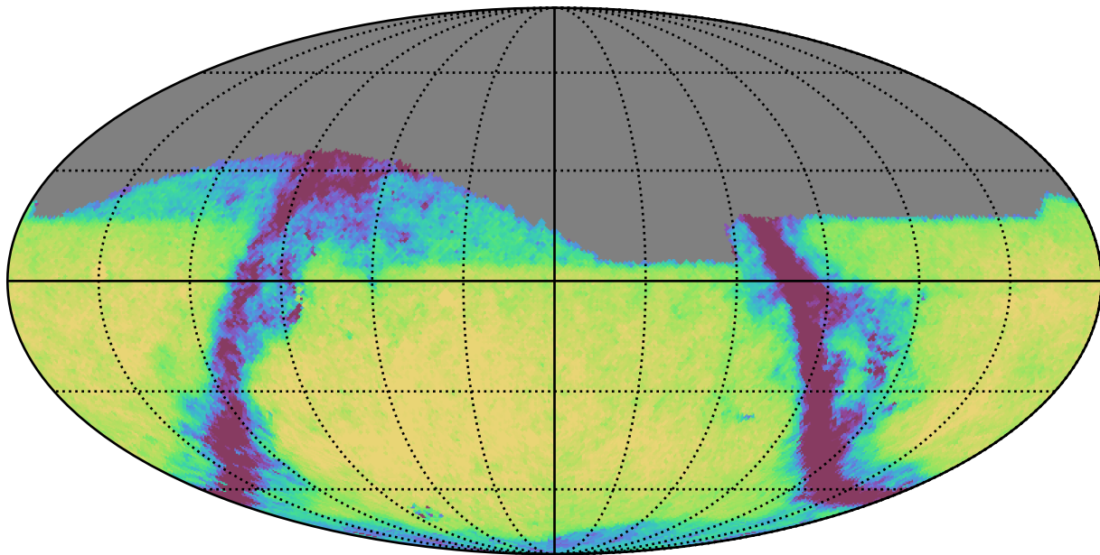
extra_ss_neo4_v3.4_10yrs Yr 1 r band: Exgal_CoaddM5
