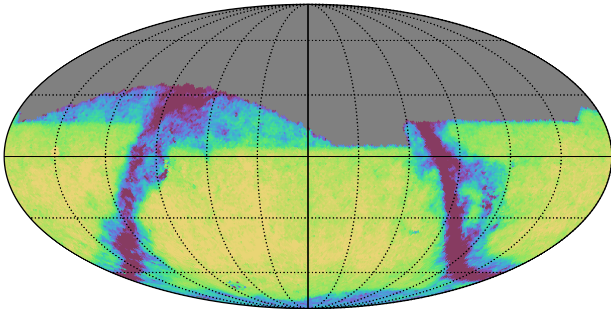
extra_ss_neo4_v3.4_10yrs Yr 1 i band: Exgal_CoaddM5
