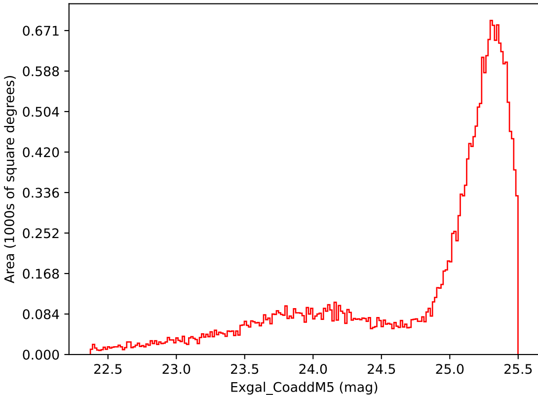
extra_ss_neo4_v3.4_10yrs Yr 1 i band: Exgal_CoaddM5
