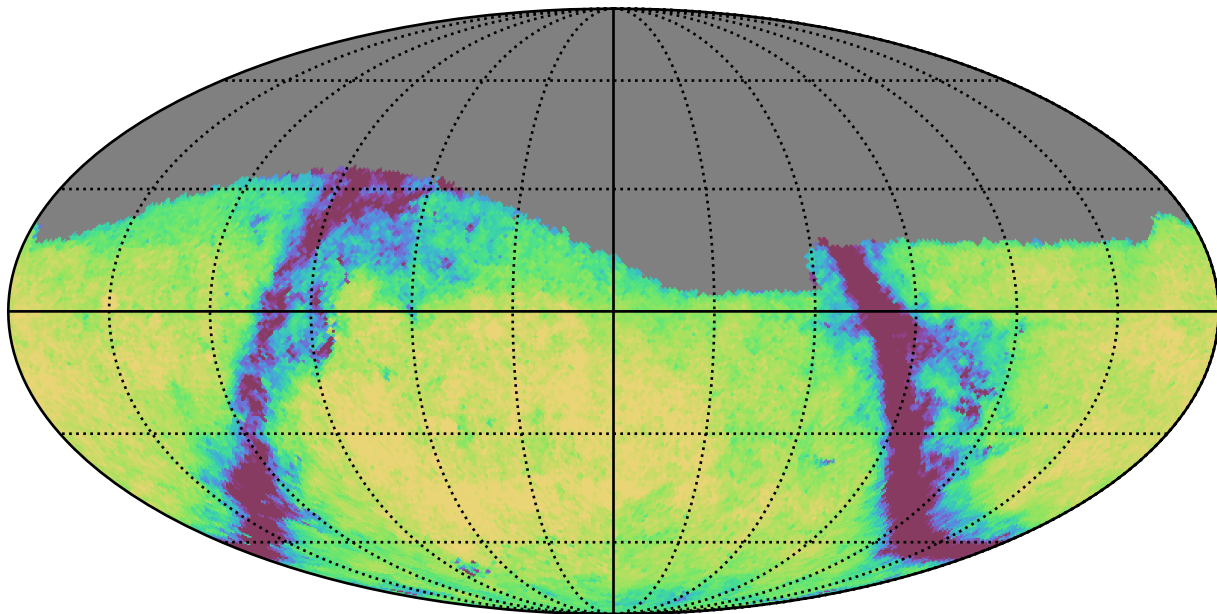
extra_ss_neo4_v3.4_10yrs Yr 1 g band: Exgal_CoaddM5
