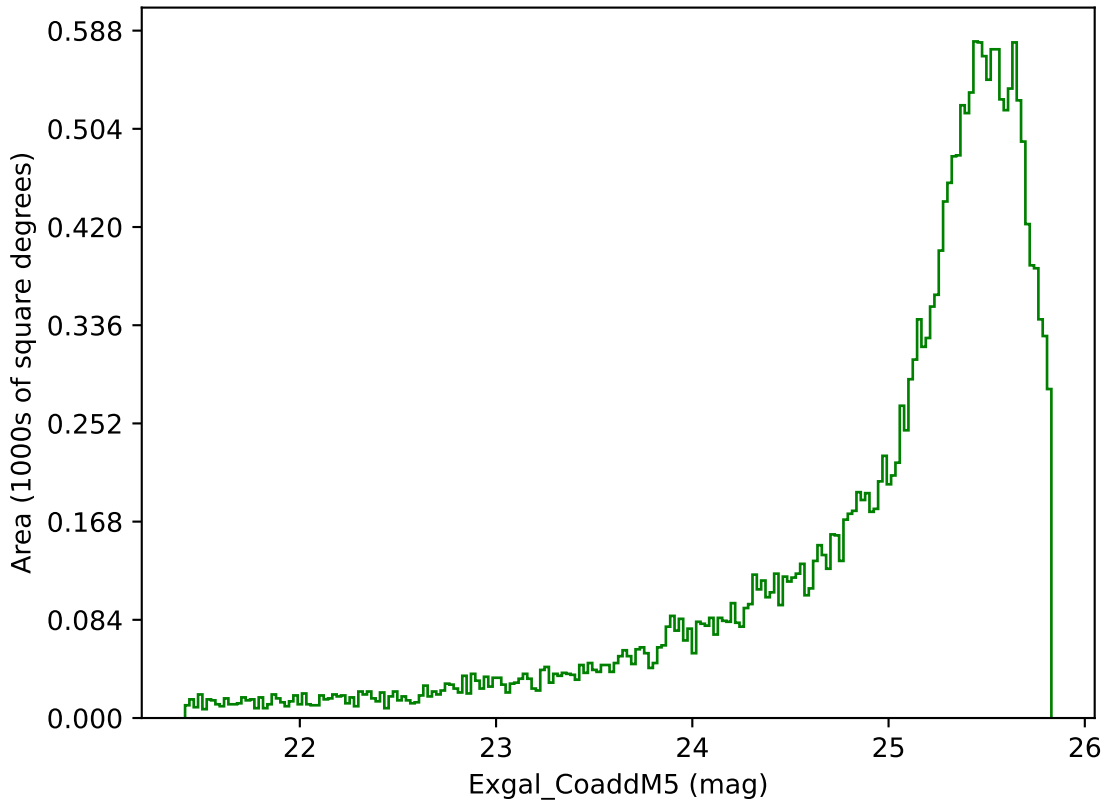
extra_ss_neo4_v3.4_10yrs Yr 1 g band: Exgal_CoaddM5
