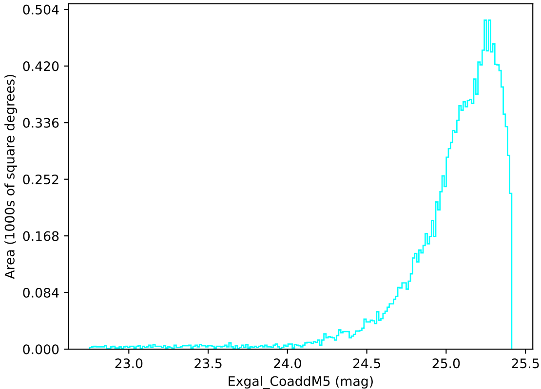
extra_ss_neo4_v3.4_10yrs WFD u band: Exgal_CoaddM5
