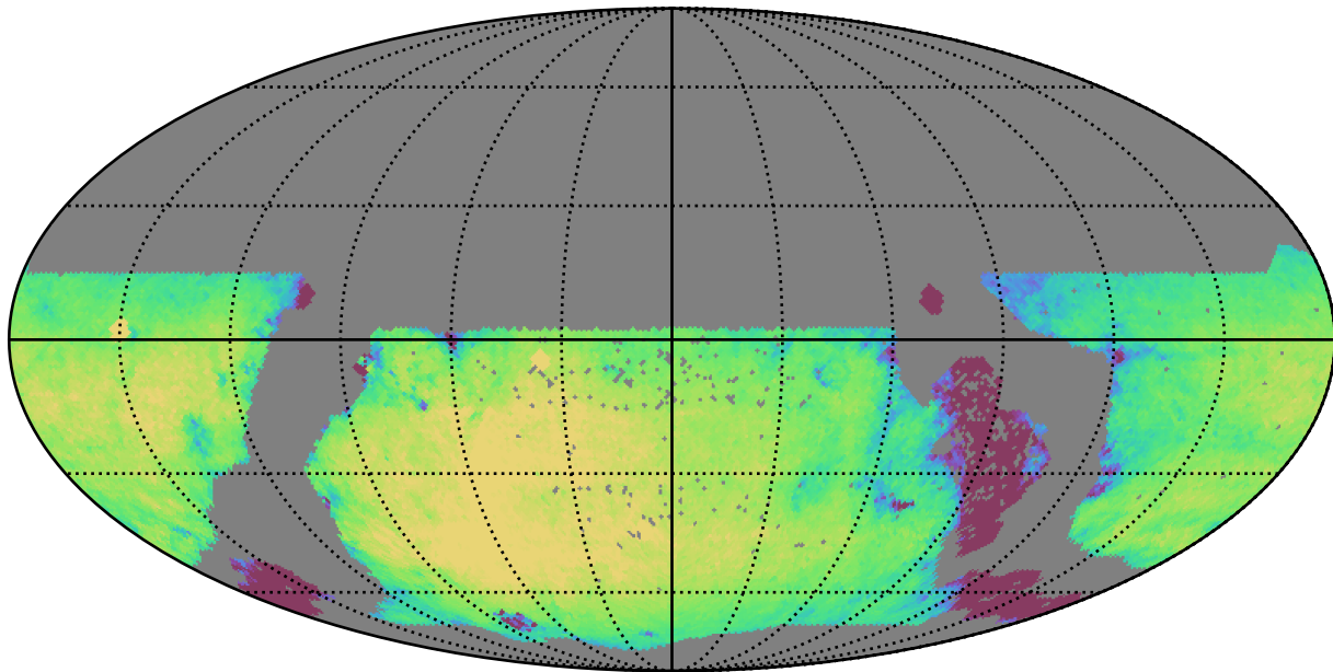
extra_ss_neo4_v3.4_10yrs WFD r band: Exgal_CoaddM5
