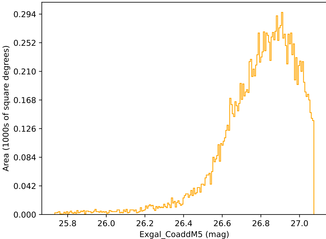
extra_ss_neo4_v3.4_10yrs WFD r band: Exgal_CoaddM5
